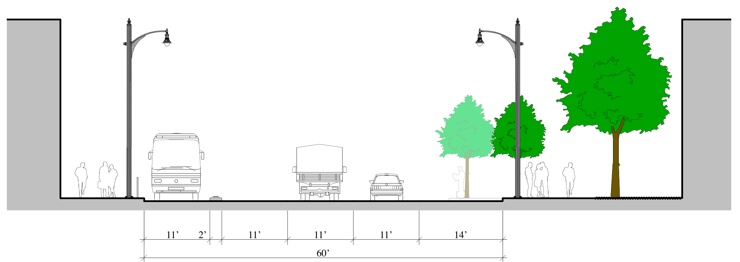
PROPOSED FIFTH AVENUE SECTION
