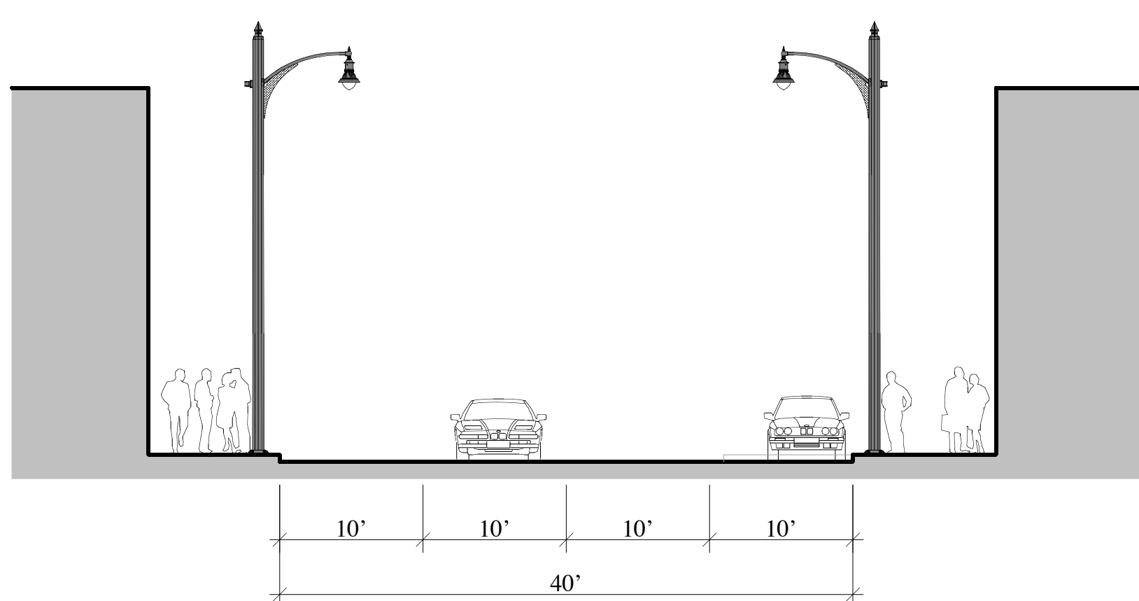
PROPOSED FORBES AVENUE SECTION
