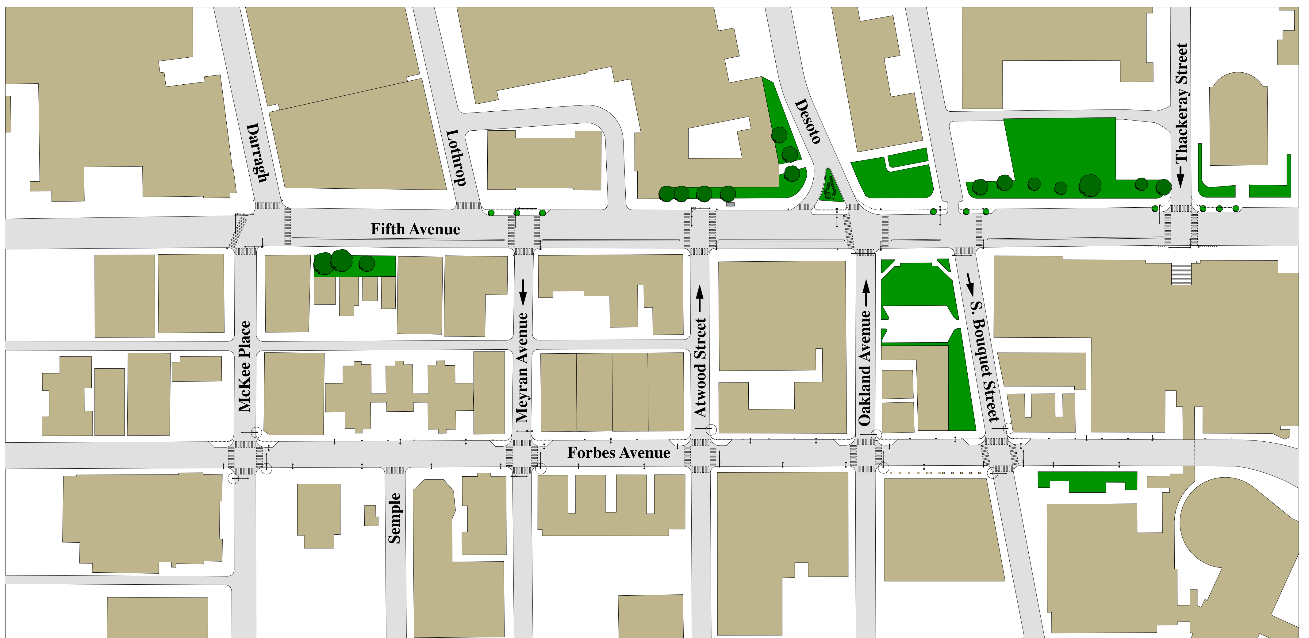
SITE PLAN
