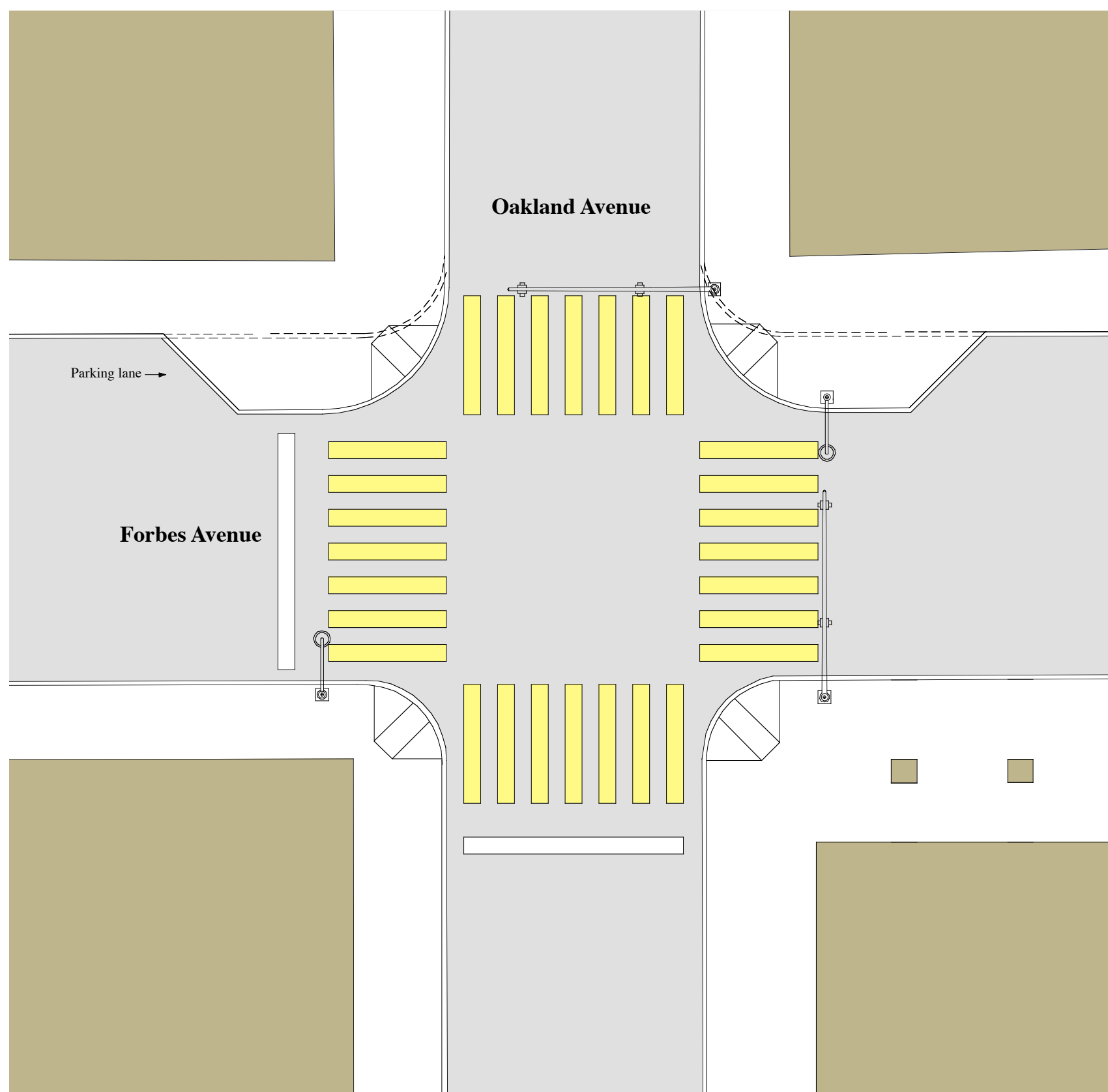
TYPICAL FORBES AVENUE INTERSECTION STRIPED CROSSWALKS AND BUMPOUTS
