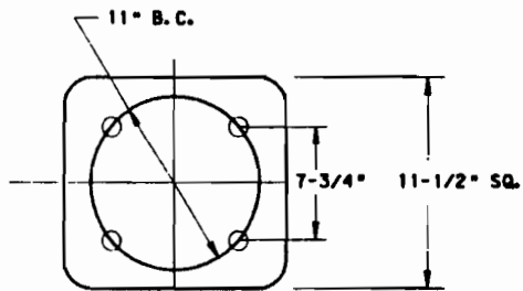
CAST STEEL BASE DETAIL
